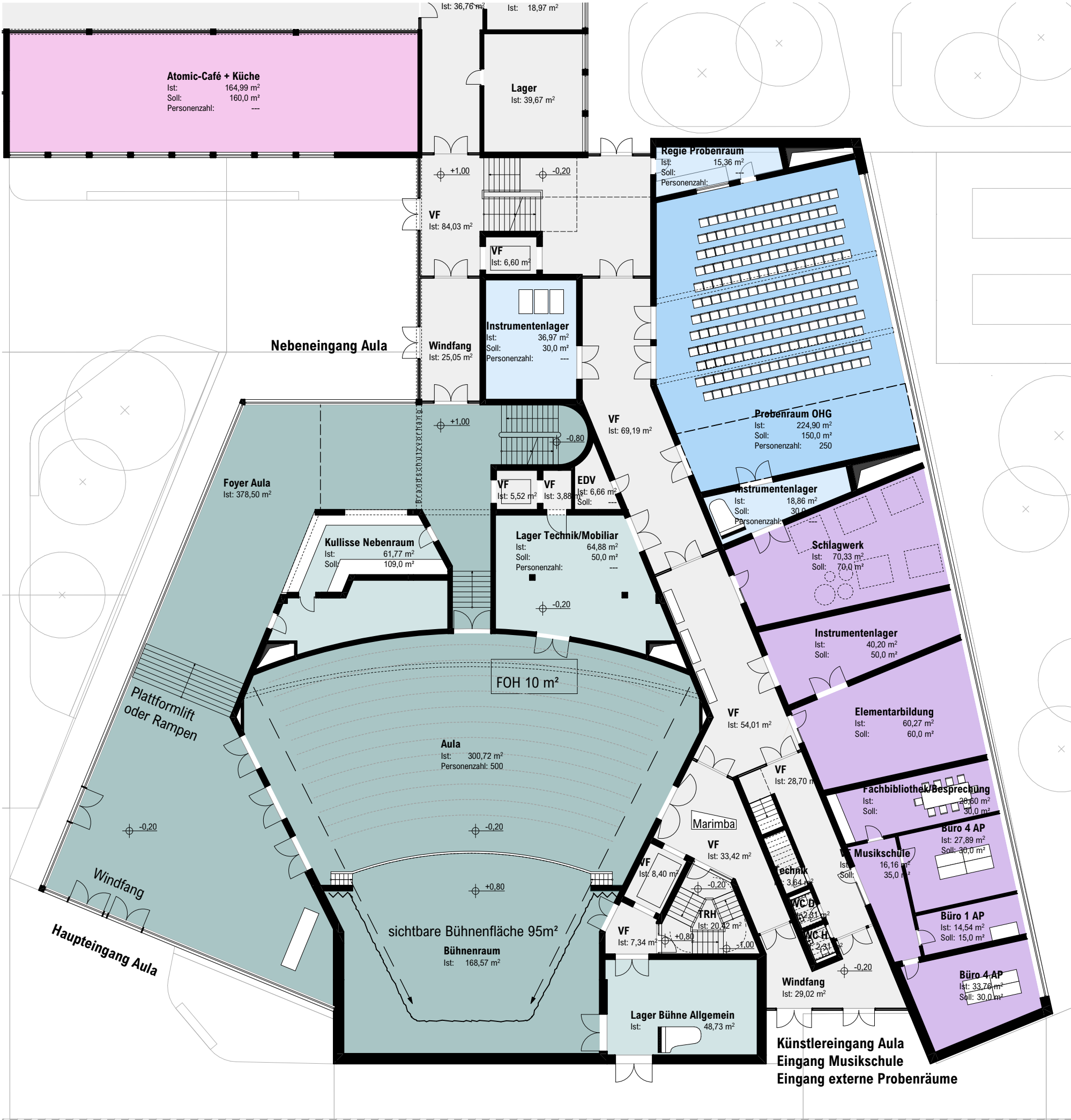
1m 5m 10m Grundriss Erdgeschoss
